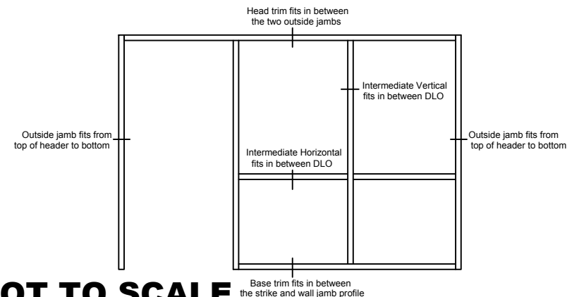
TRIM CUTTING DIAGRAM COMMENDED FIELD CUTTING TO FIT)
